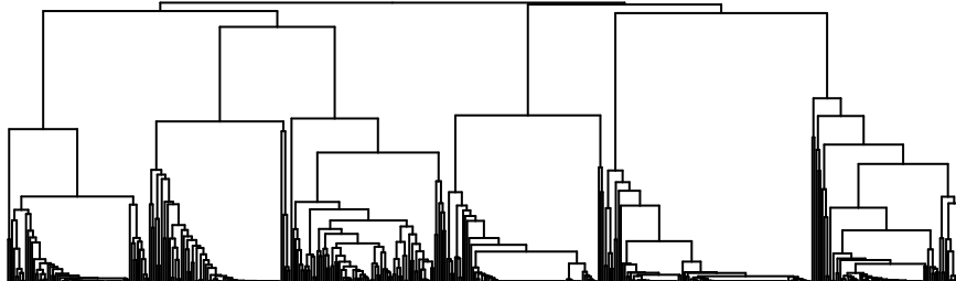
consensus matrix k=6
